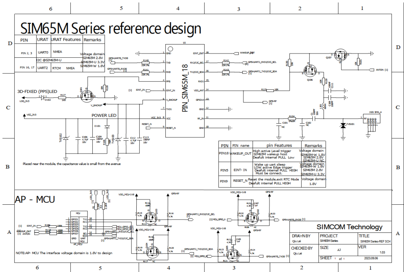
Figure 33: Refer schematic
