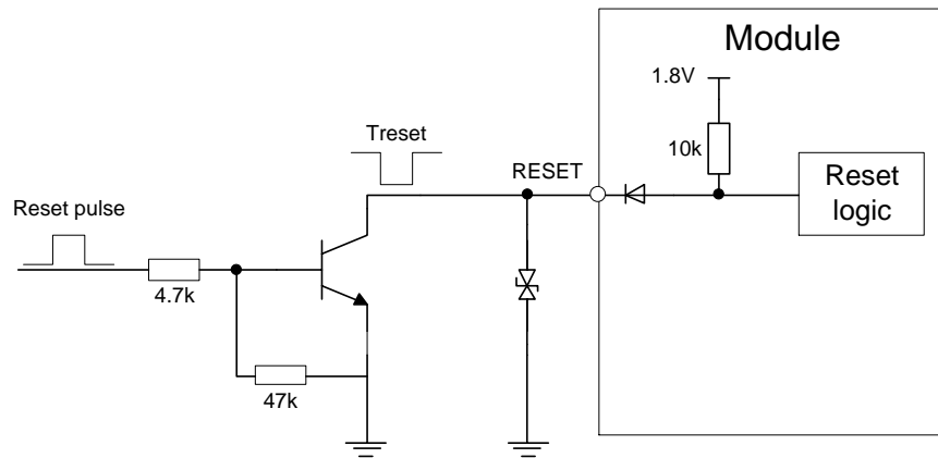
Figure 12: RESET recommended circuit
