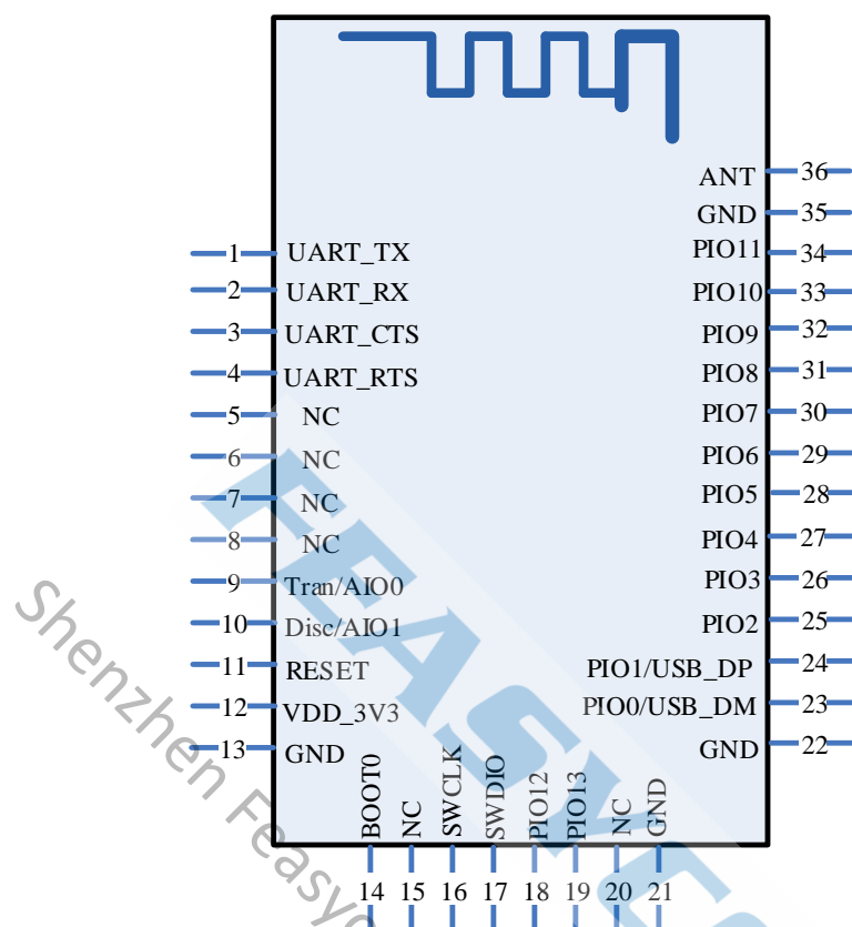
Figure 1: FSC-BT836BG PIN Diagram
